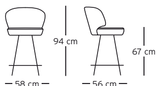
Barstuhl (Drahtuntergestell) Bar stool (wire base)
